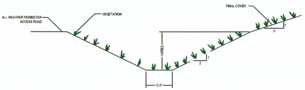
PERIMETER DRAINAGE CHANNEL
